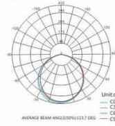
Light distribution curve
